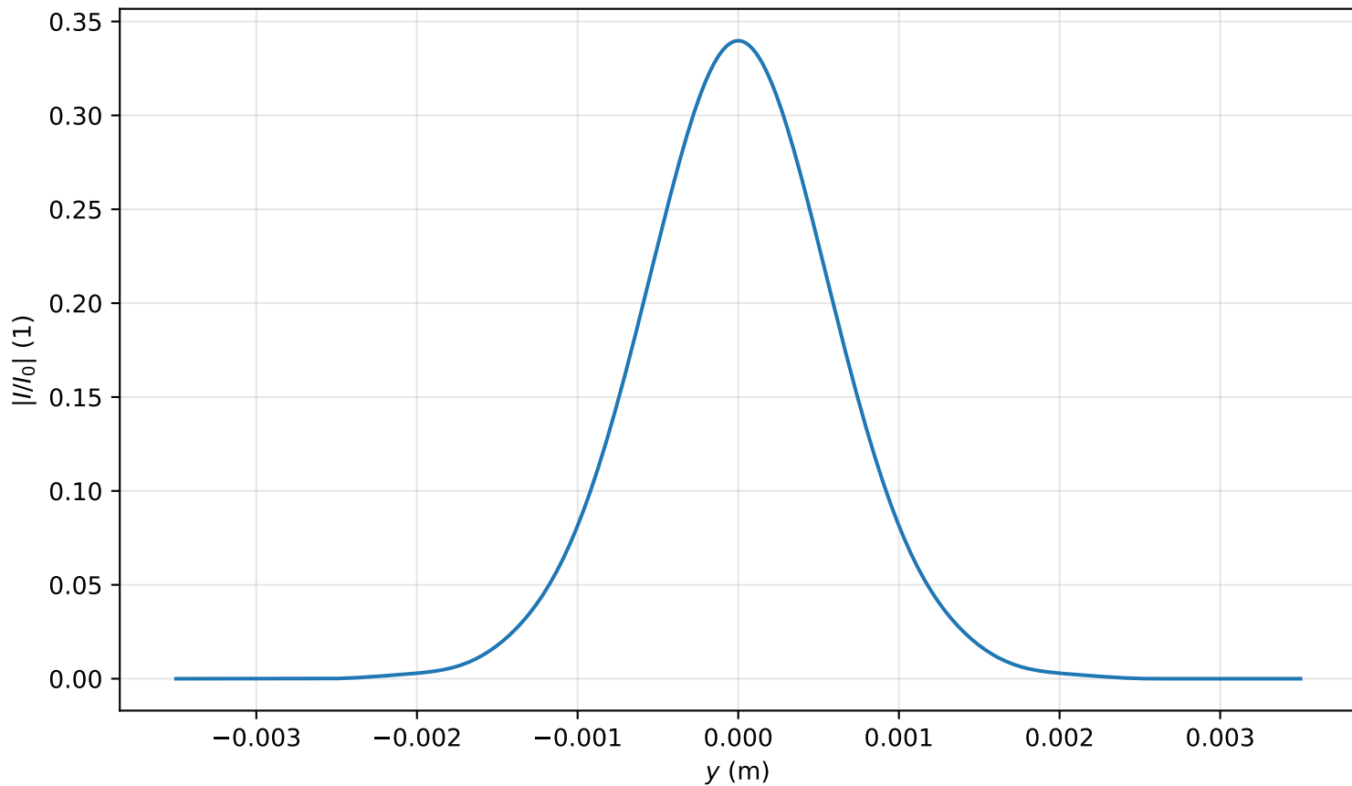
Intensity profile I(x=0, y, z=3.901)/I_0 , P_{in}=0.4P_{cr} , artificial time
